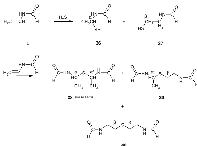
Scheme 11 Simple and multiple addition reactions of \text{H}_2\text{S} to 1
