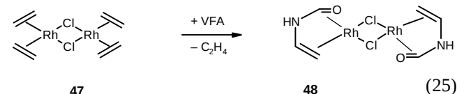
Scheme 12 Cationic oligomerisation of 1 and possible chain termination reactions
